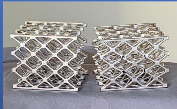
Pre-test lattice compression sample (left) and post-test samples (right) that were loaded from the side
