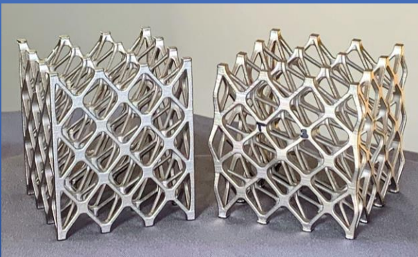
Pre-test lattice compression sample (left) and post-test samples (right) that were loaded from the top
